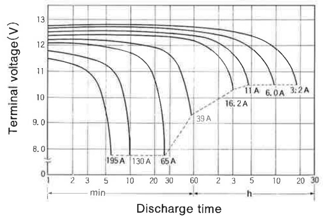
Discharge characteristics (0°C (32°F))
