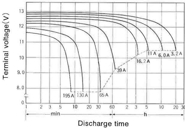
Discharge characteristics (25°C (77°F))
