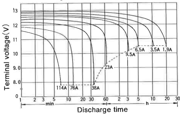
Discharge characteristics(25°C(77°F))
