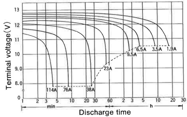
Discharge characteristics(0°C(32°F))
